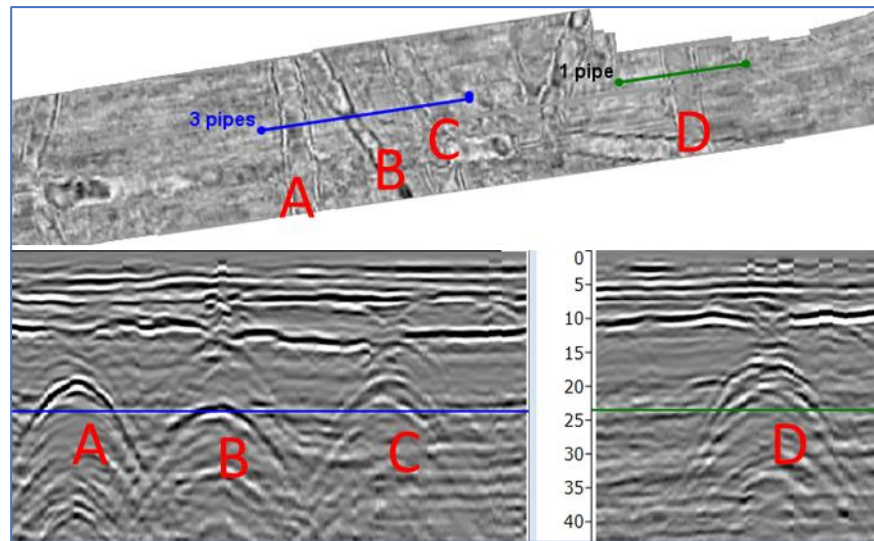
Figure 115 Top: C-scan with marked 2D cuts across four linear targets. Bottom 2D-views of the cuts marked in C-scan. Horizontal lines in the 2D views shows the depth/time of the C-scan
