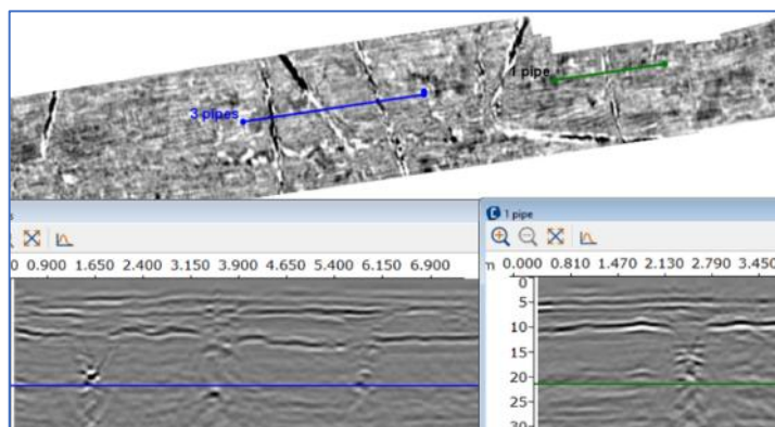
Figure 118 Result of 3D-migration with velocity set to 80 m/ \mu s
