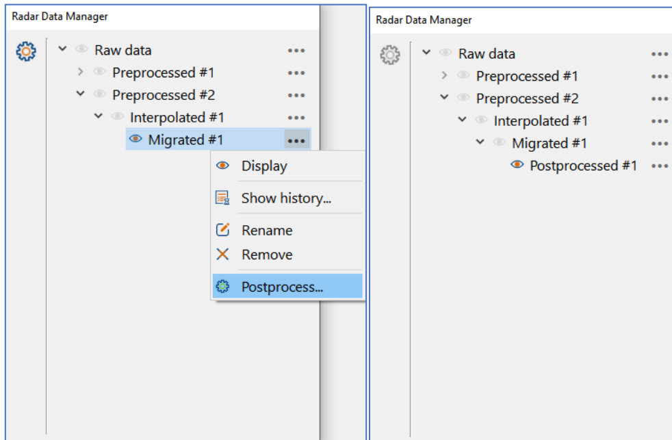
Figure 63 Adding the first branch with Postprocessing procedures
