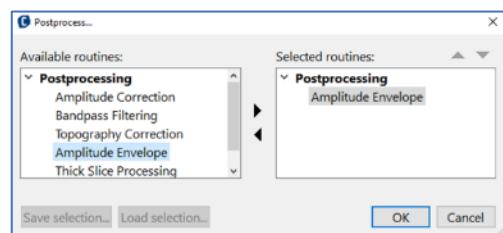
Figure 113 post-processing routines
