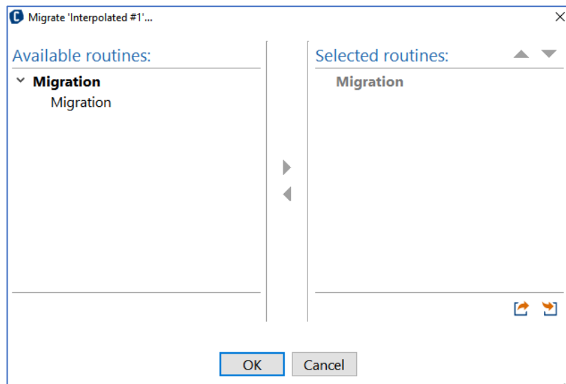
Figure 55 Migration stage
