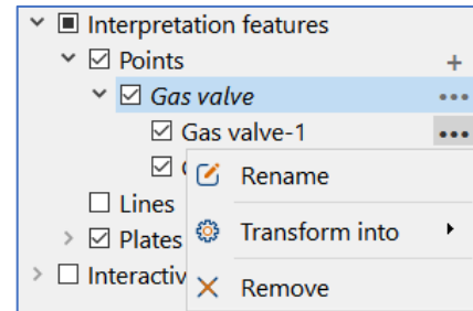
Figure 71 Rename/Transform commands
