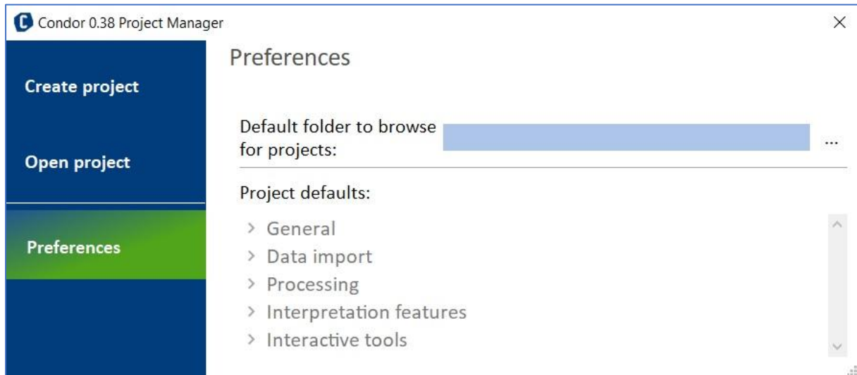
Figure 20 Preferences window
