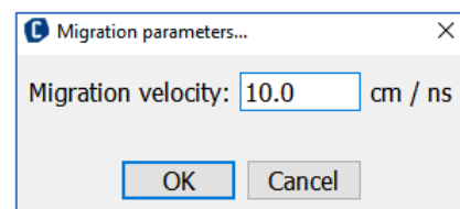
Figure 58 Migration parameters
