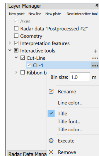
Figure 77 Cut-line parameters
