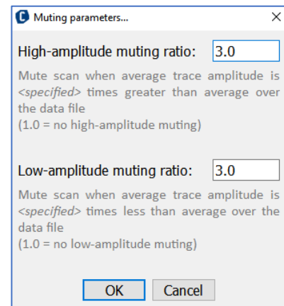
Figure 49 Muting parameters
