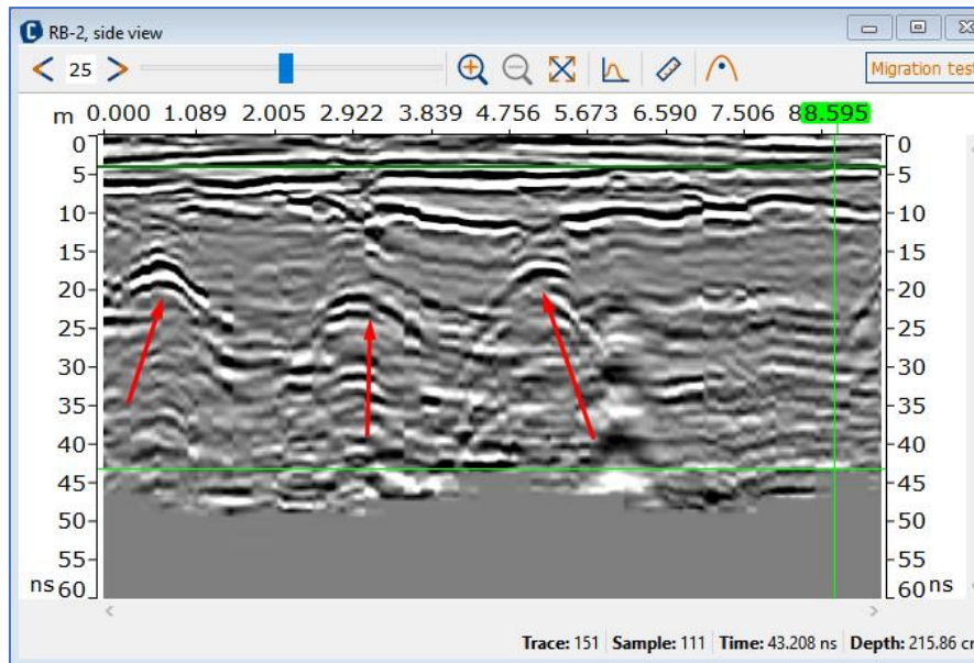
Figure 56 Hyperbola reflections from point objects
