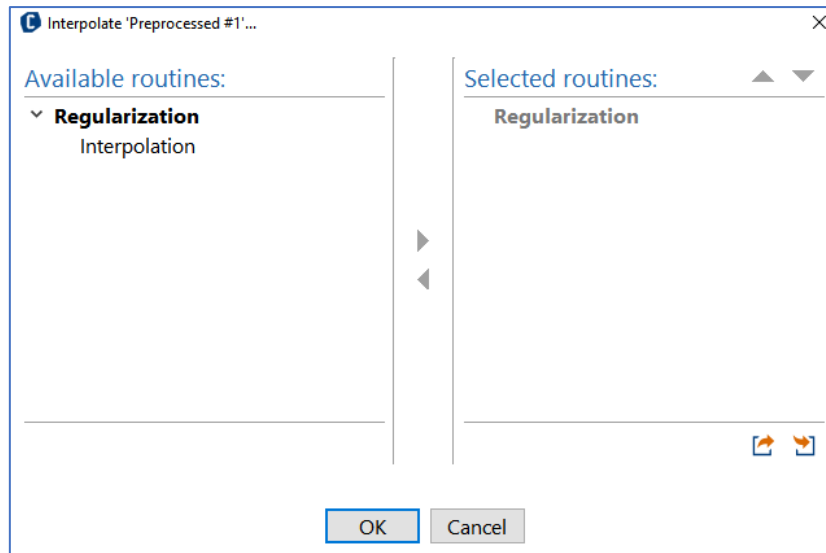
Figure 53 Regularization stage
