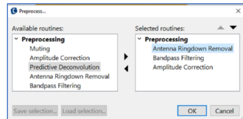
Figure 109 Pre-processing routines
