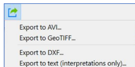
Figure 19 Exports options
