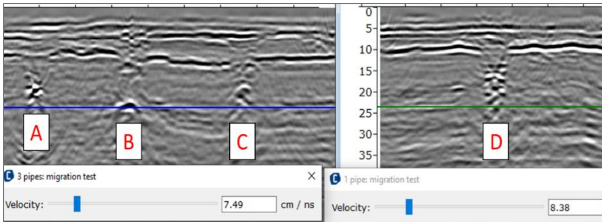
Figure 117 Test migration of the two radargrams from figure 1, left migrated with 75 m/ \mu s and right with 84 m/ \mu s
