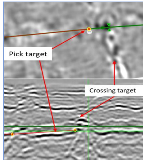
Figure 122 Picking a target along the horizontal outline in top view while crossing under a target coming in from 90 degrees.
